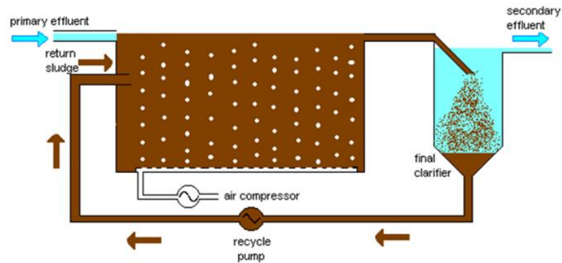
Activated Sludge Process
