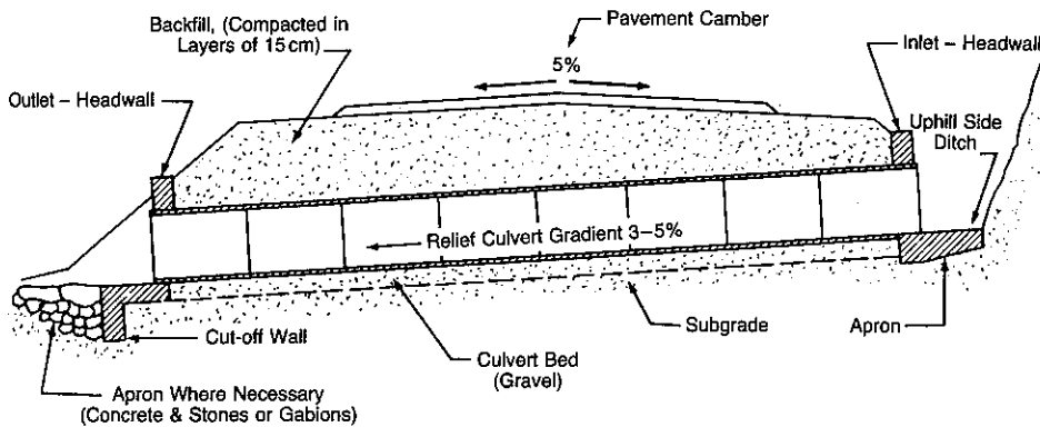
Figure 11.4 Pipe culvert (ref. 4).
