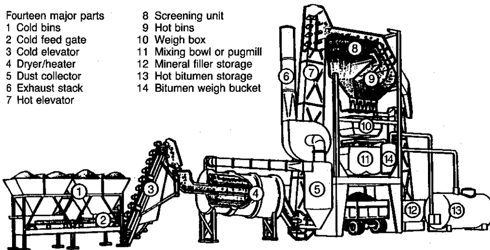
Figure 15.4 Batch mixer (ref. 4).
