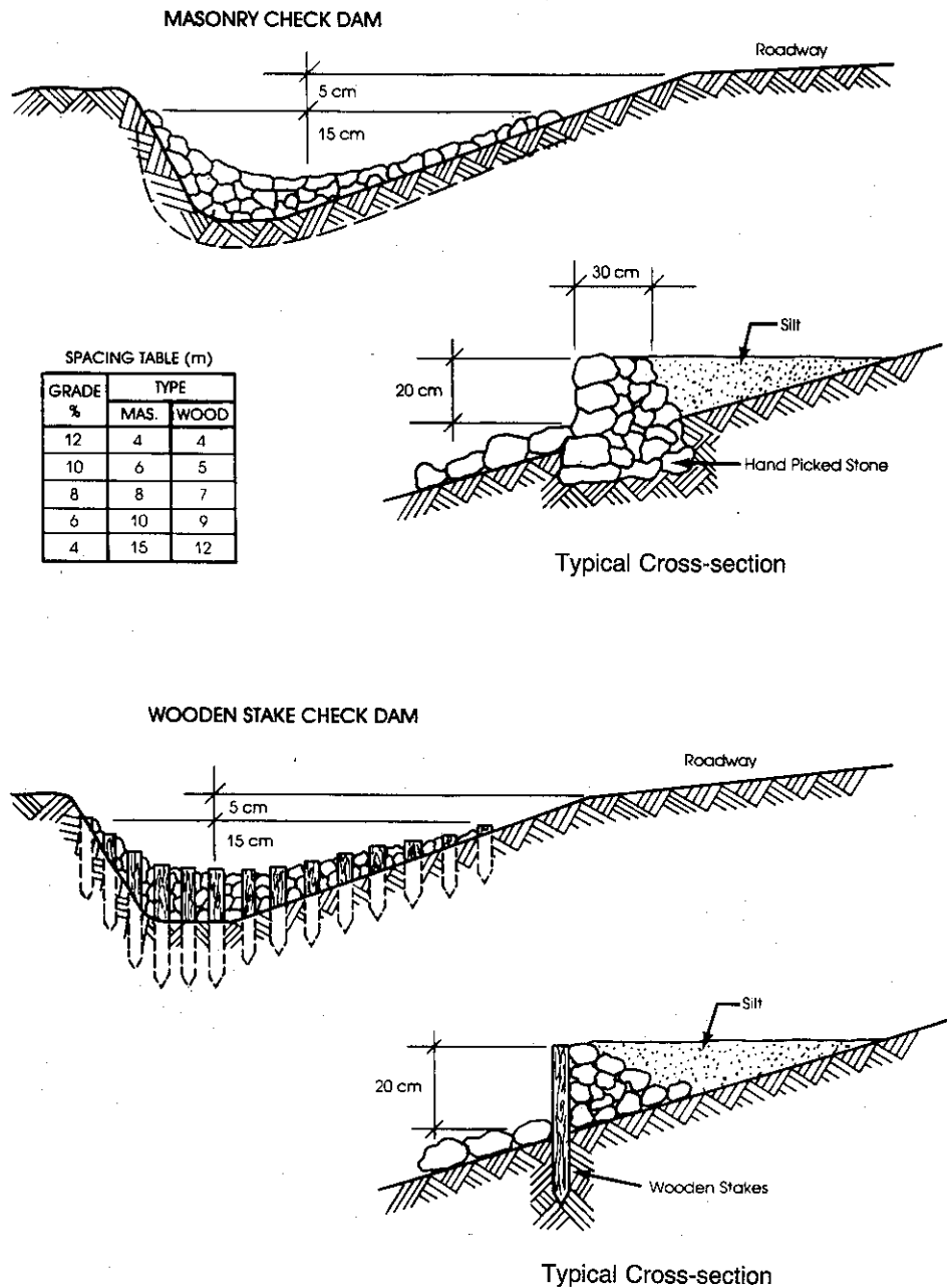
Figure 11.12 Ditch checks (ref. 4).
