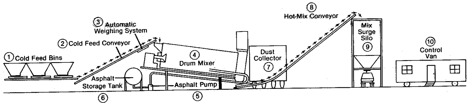
Figure 15.5 Drum mixer (ref. 5).
