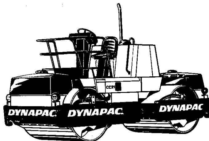
Figure 14.5 Self-propelled, vibratory, smooth steel-wheeled roller.
