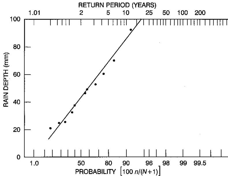
Figure 10.2 Extreme probability plot (ref. 1).
