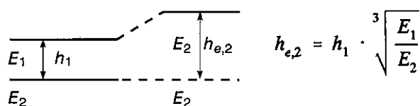
Figure 16.6 Two-layer system.
