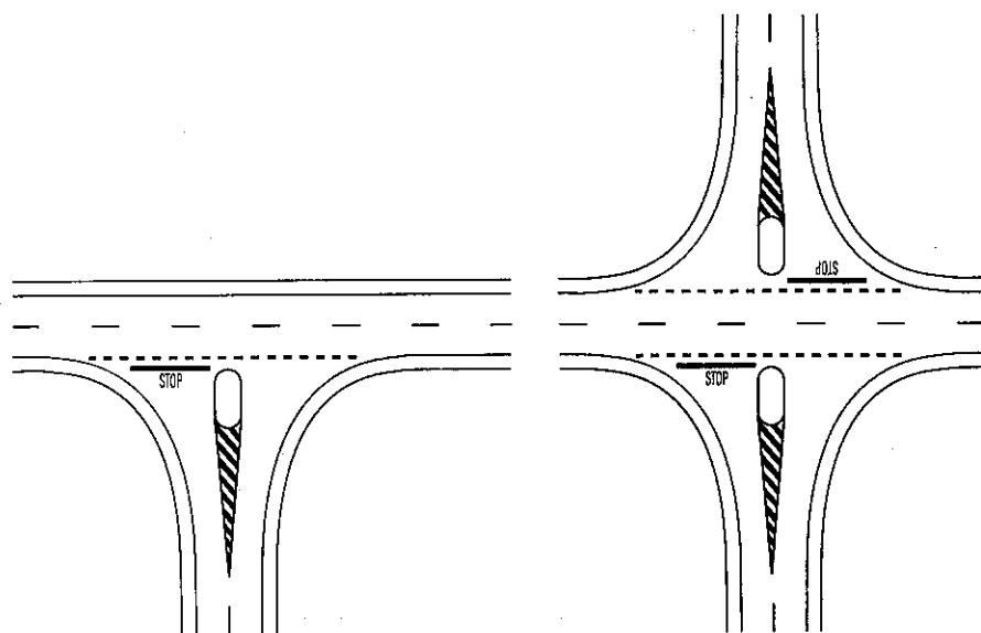
Figure 8.8 Intersection layouts for low-volume roads with light turning traffic from the major to the minor road (ref. 2).
