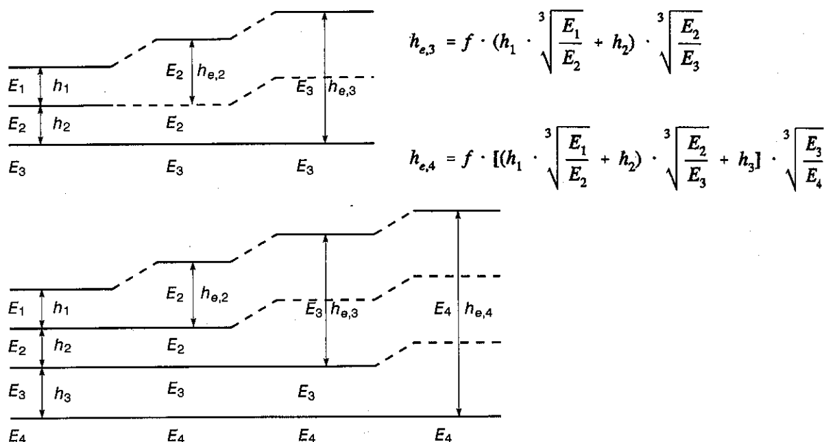
Figure 16.7 Three- and four-layer systems.
