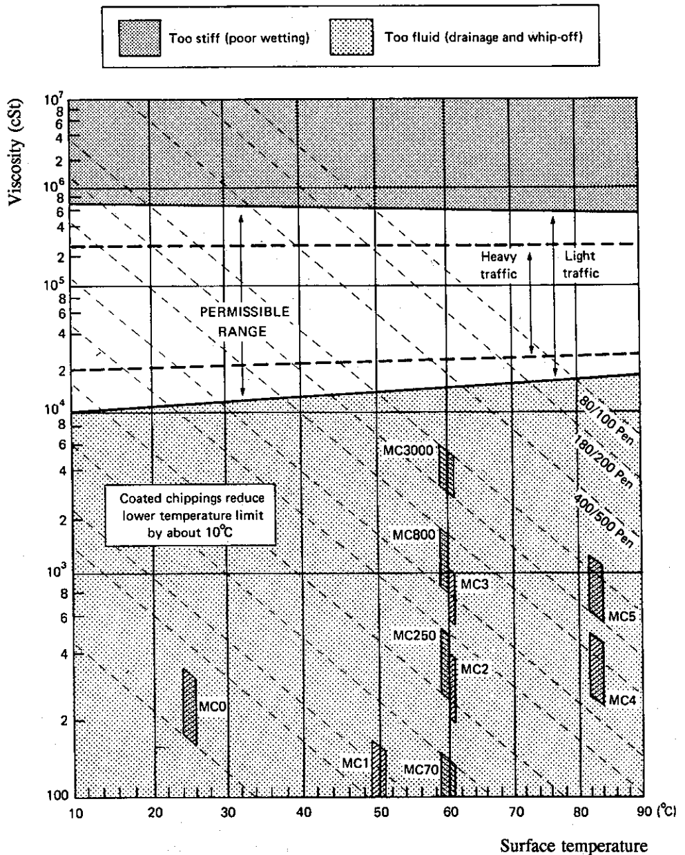
Figure 15.2 Choice of binder for surface dressing (TRRL Overseas Road Note 3, ref. 2).
