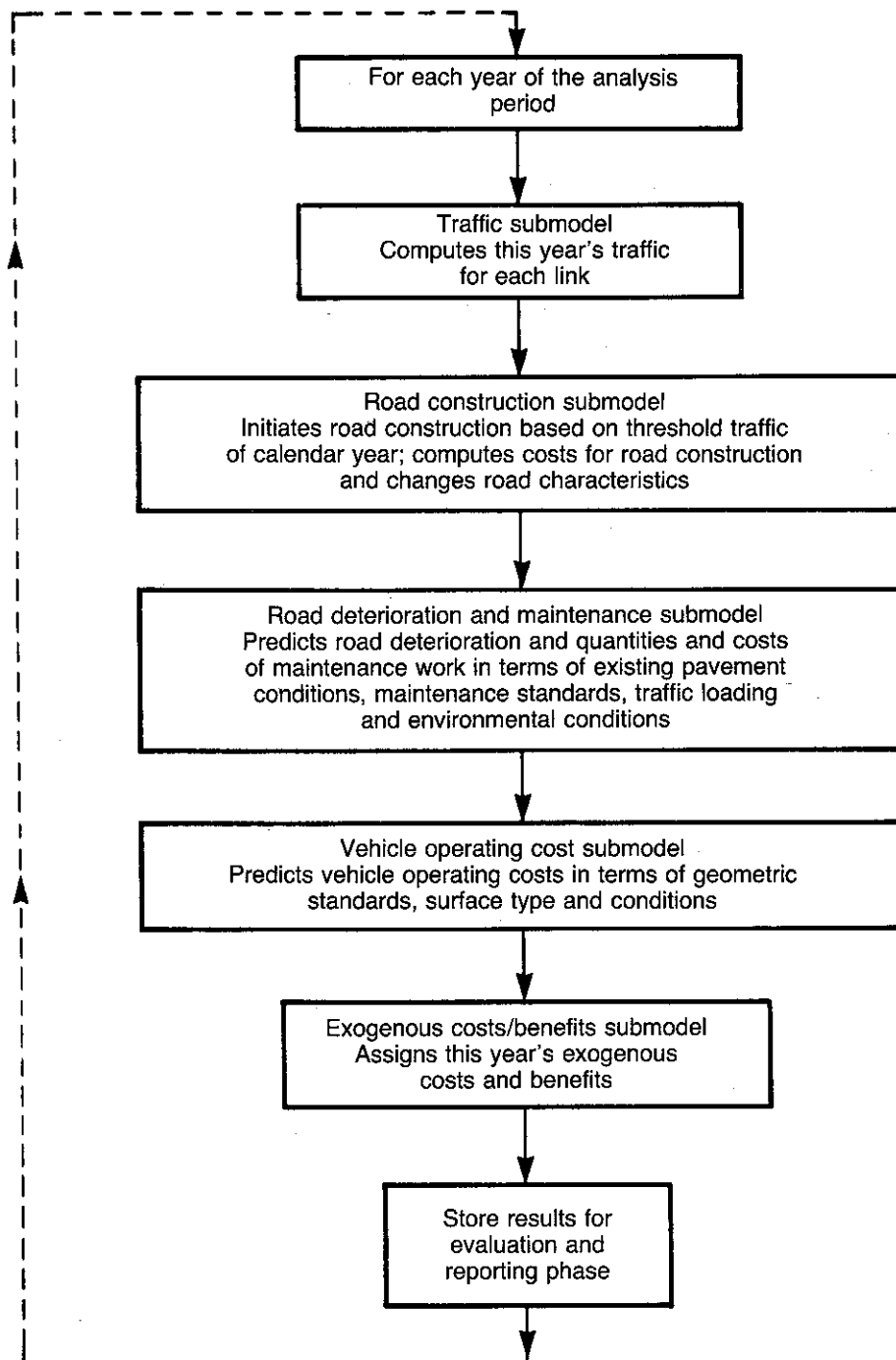
Figure 4.1 Simulation of a link alternative (ref. 4).
