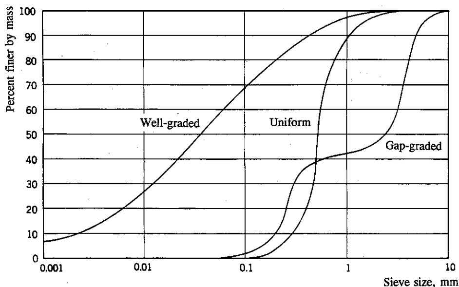
Figure 12.7 Particle size distribution curves.
