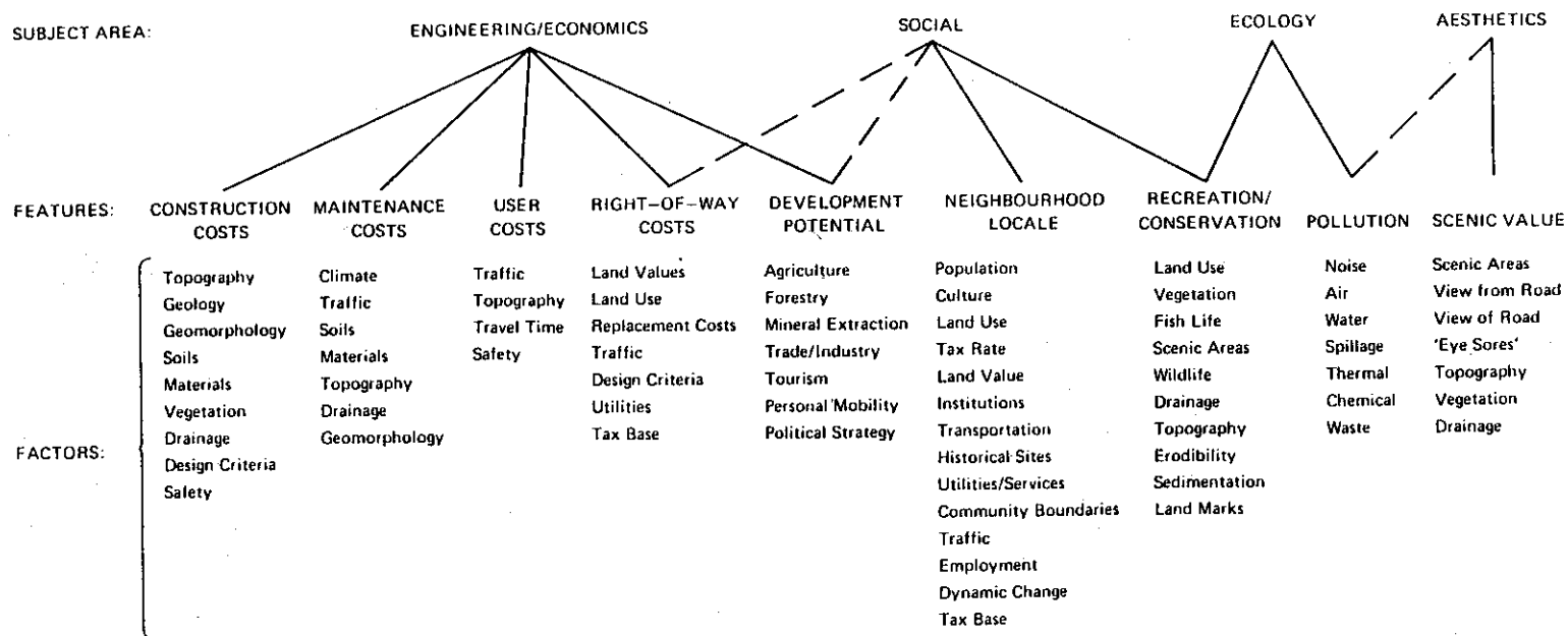
Figure 8.5 Factors affecting road alignment selection (TRRL Supplementary Report 279, ref. 5).
