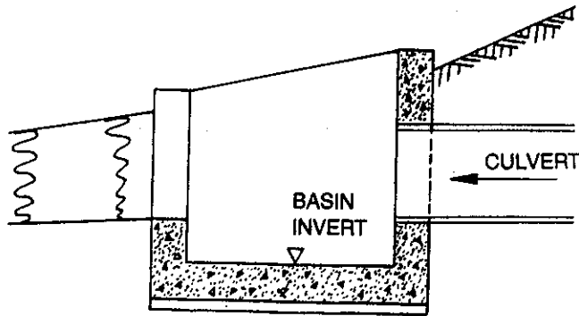
Figure 20.8 Outfall basin (ref. 2).
