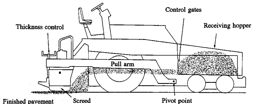
Figure 15.6 Asphalt paver (ref. 5).
