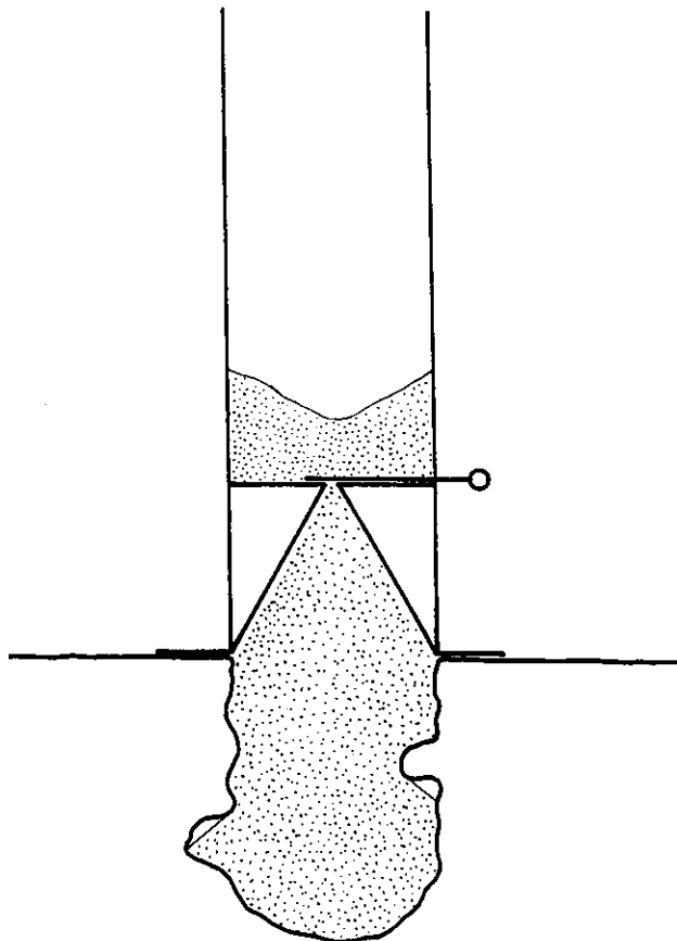
Figure 12.9 Sand cone.
