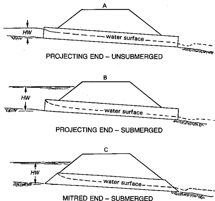
Figure 11.6 Inlet control (Transportation Research Board, ref. 3).
