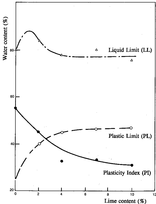
Figure 14.8 Effect of the addition of lime on a London clay (ref. 5). (Crown copyright; reproduced with the permission of the Controller of HMSO.)
