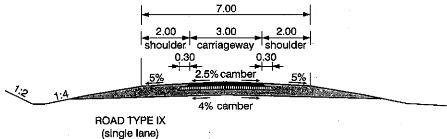
Figure 9.2 Typical cross-section (ref. 3).
