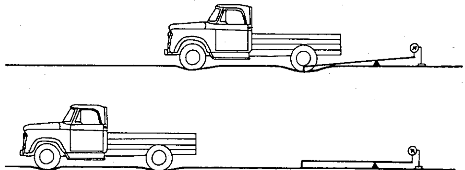
Figure 16.8 Benkelman beam measurement.
