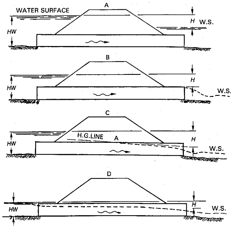
Figure 11.7 Outlet control (Transportation Research Board, ref. 3).
