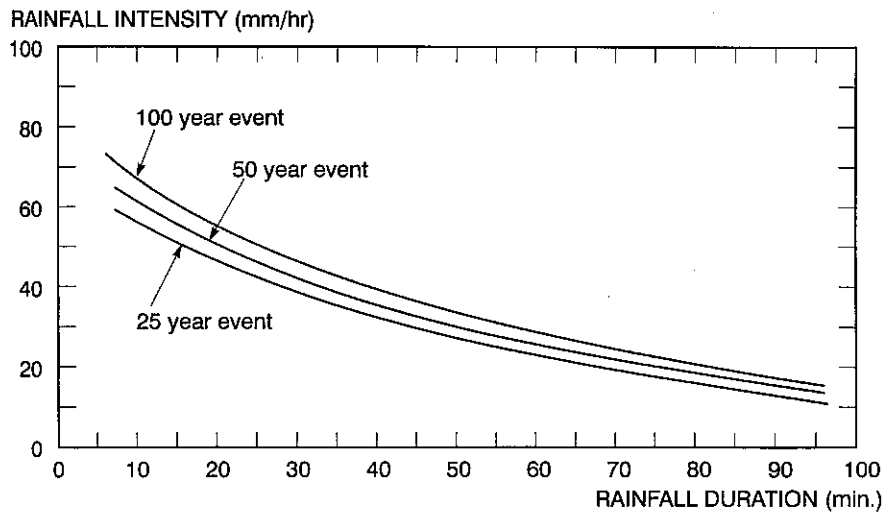
Figure 10.3 Intensity-duration curves.
