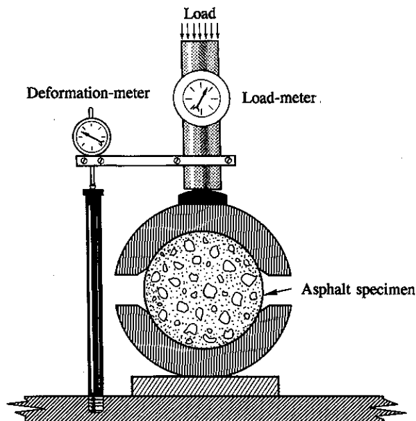
Figure 15.7 Marshall testing machine.
