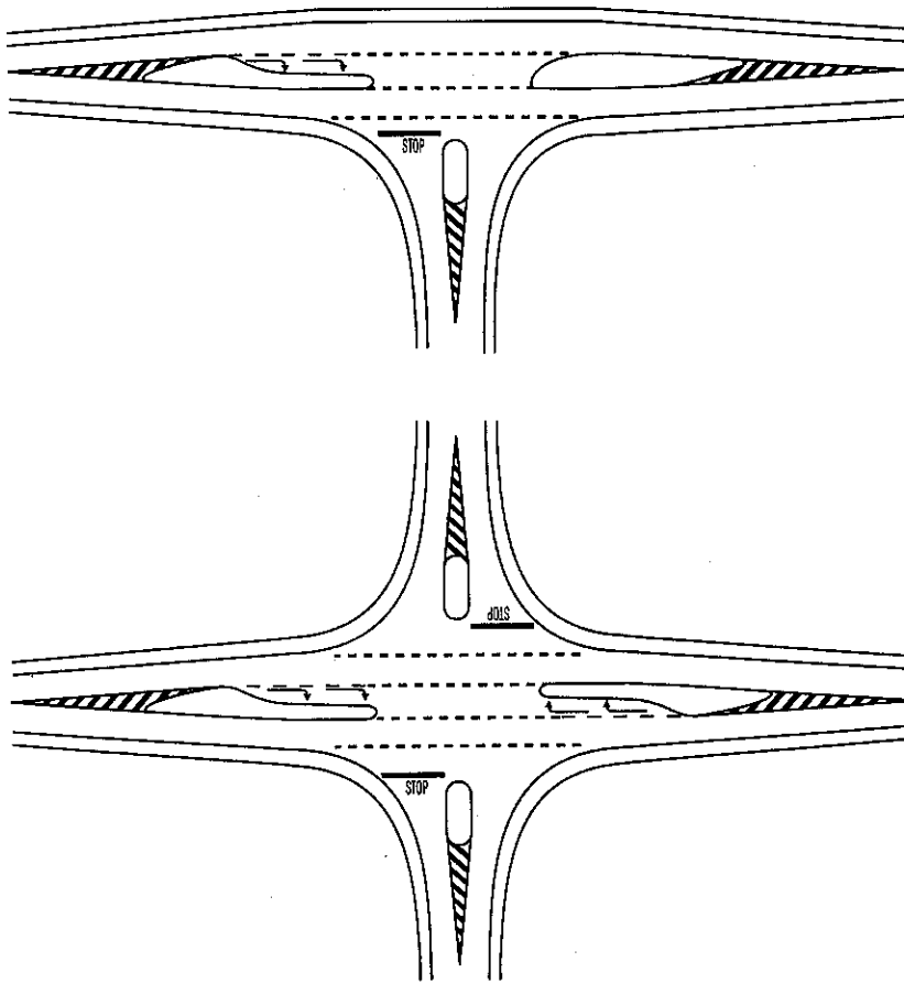
Figure 8.9 Channelized intersection layouts (ref. 2).
