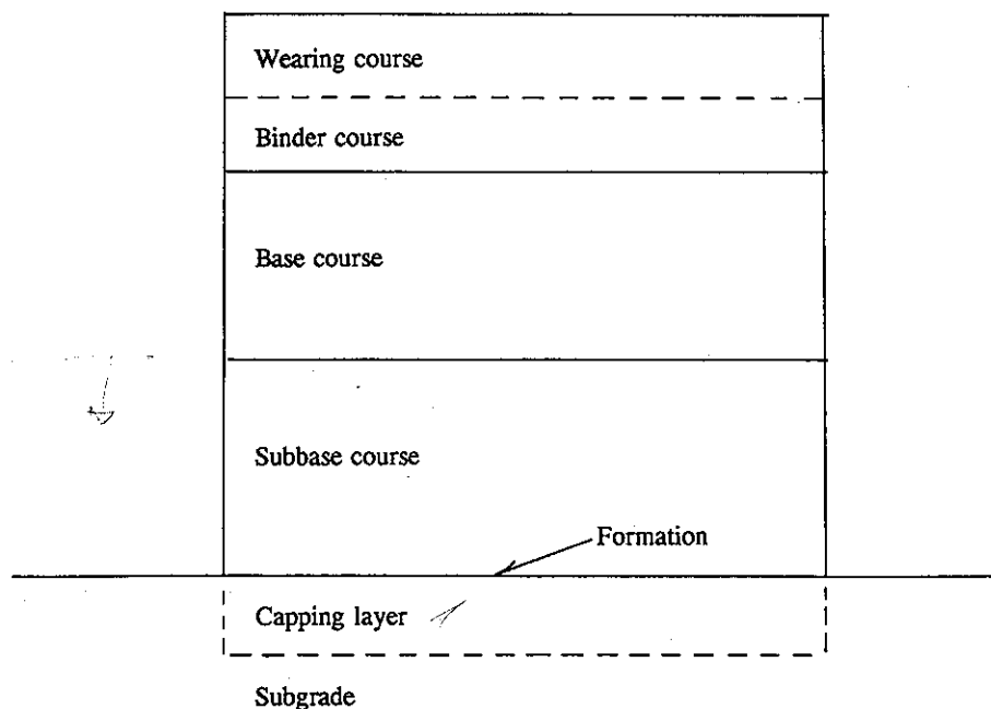
Figure 14.7 Terms used for the different pavement layers.
