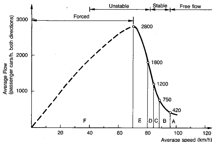
Figure 7.1 Speed–flow diagram.
