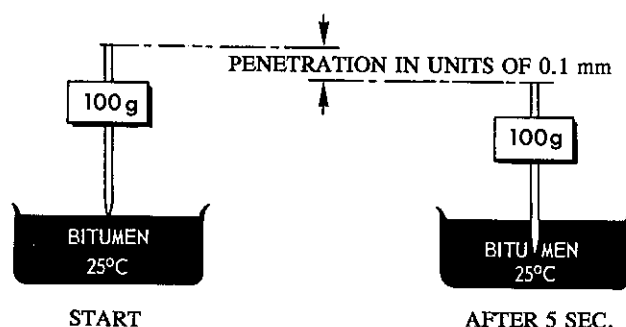
Figure 15.1 Penetration test.
