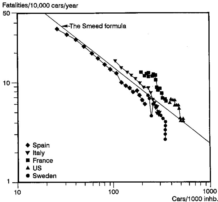
Figure 6.2 Actual development in F/M as a function of M/I for selected industrialized countries (1970–85) compared with Smeed's formula with k = 3 \times 10^{-4} .
