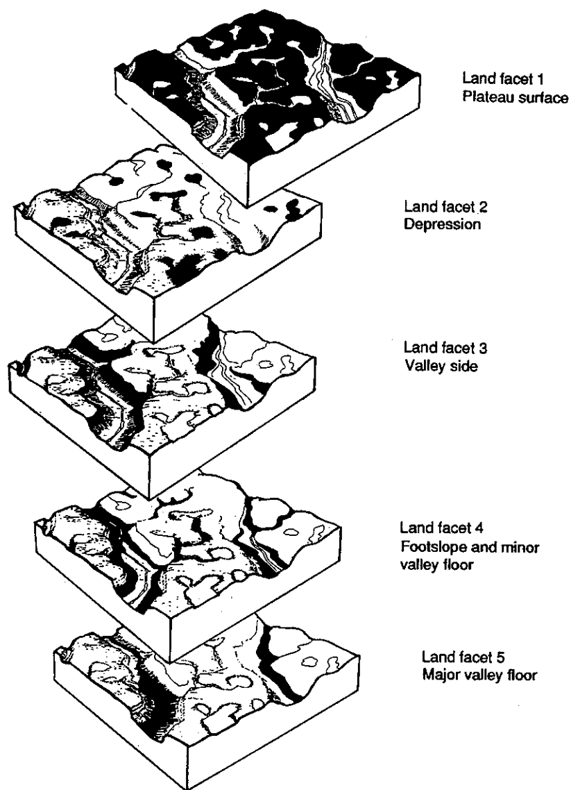
Figure 12.4 Block diagram of a land system with five land facets (ref. 2). (Crown copyright; reproduced with the permission of the Controller of HMSO.)
