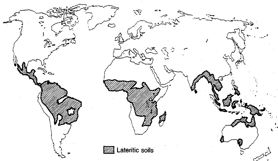
Figure 13.1 Distribution of lateritic soils (ref. 4).
