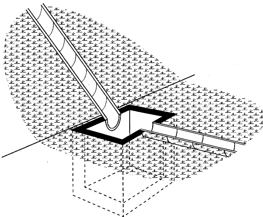
Figure 11.2 Chute outlet.
