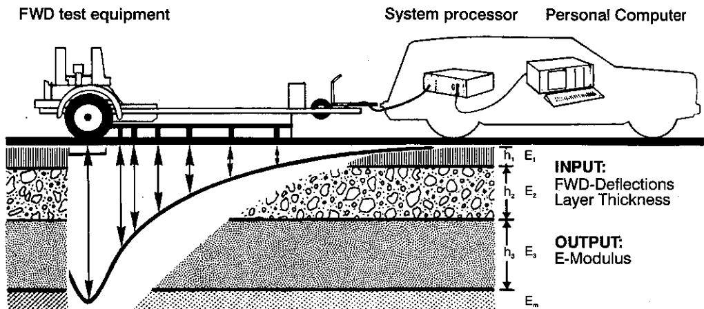
Figure 16.5 Falling weight deflectometer.
