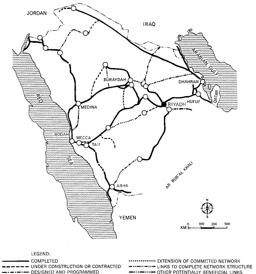
Figure 2.3 Existing and potential new highway links.
