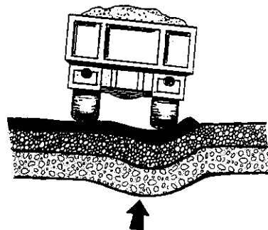
Figure 20.2 Edge subsidence (ref. 2).
