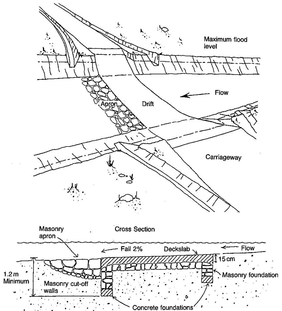
Figure 11.3 Drift (copyright International Labour Organisation) (ref. 1).
