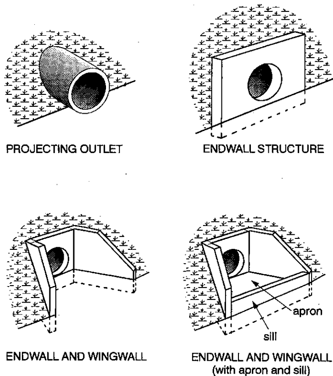
Figure 11.5 Types of culvert outlets.
