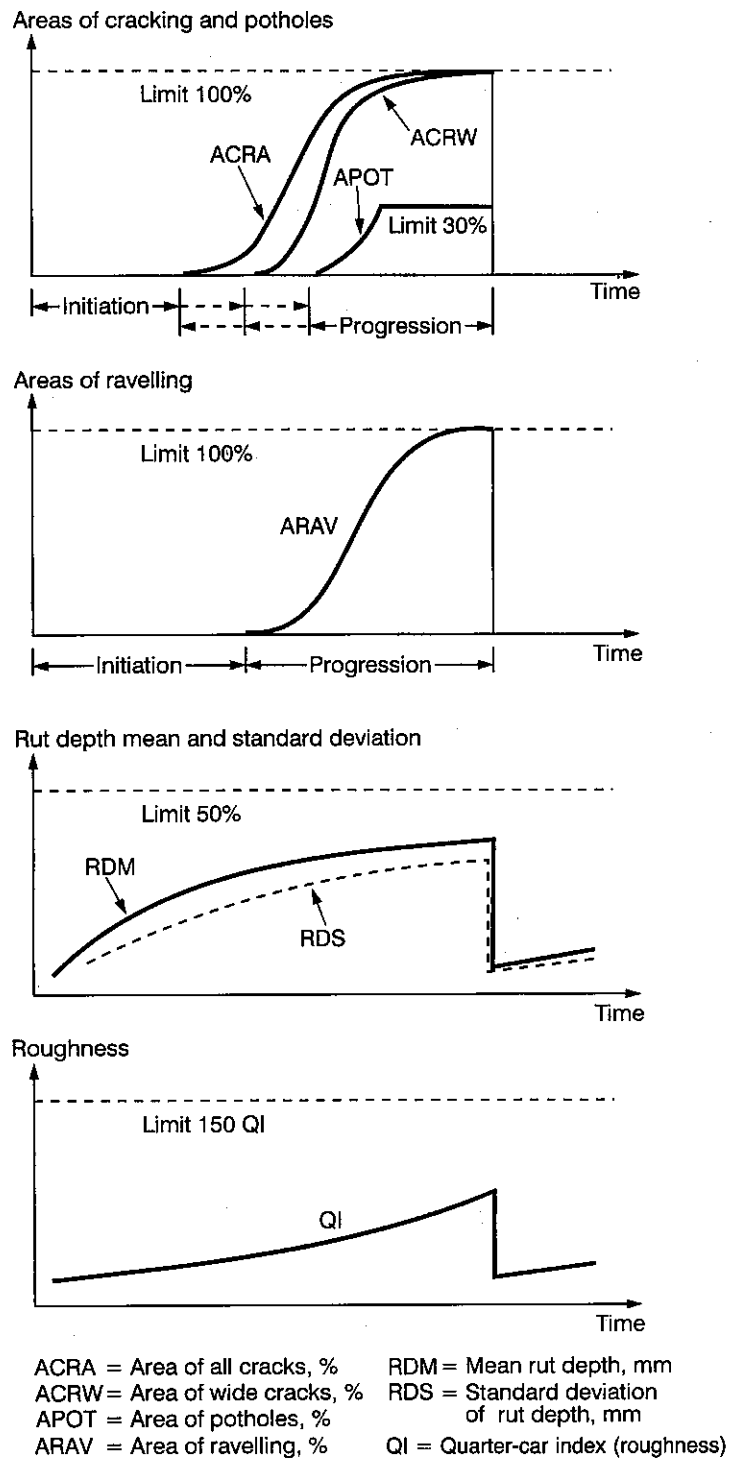
Figure 4.2 Pavement distress prediction (ref. 4).
