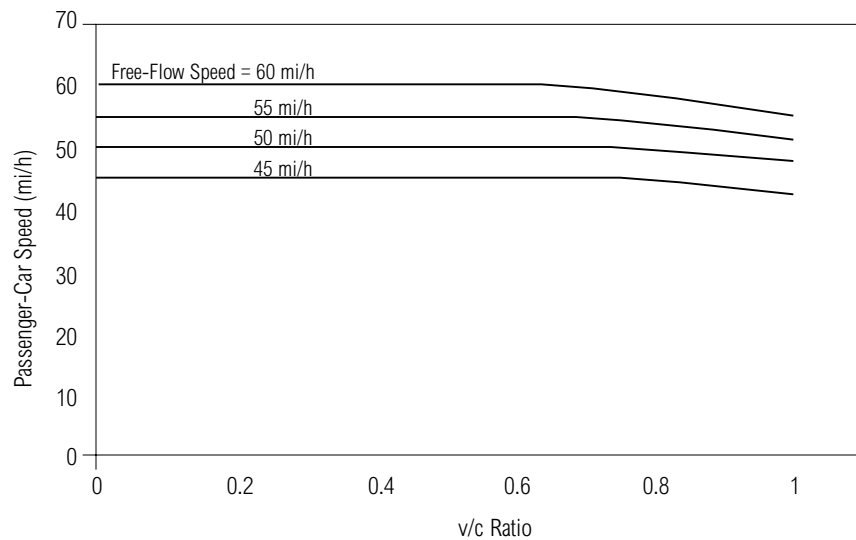
EXHIBIT 21-12. EFFECT OF v/c RATIO ON MEAN SPEED
