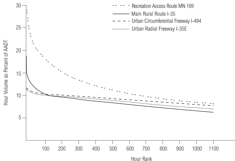
EXHIBIT 8-8. RANKED HOURLY VOLUMES
