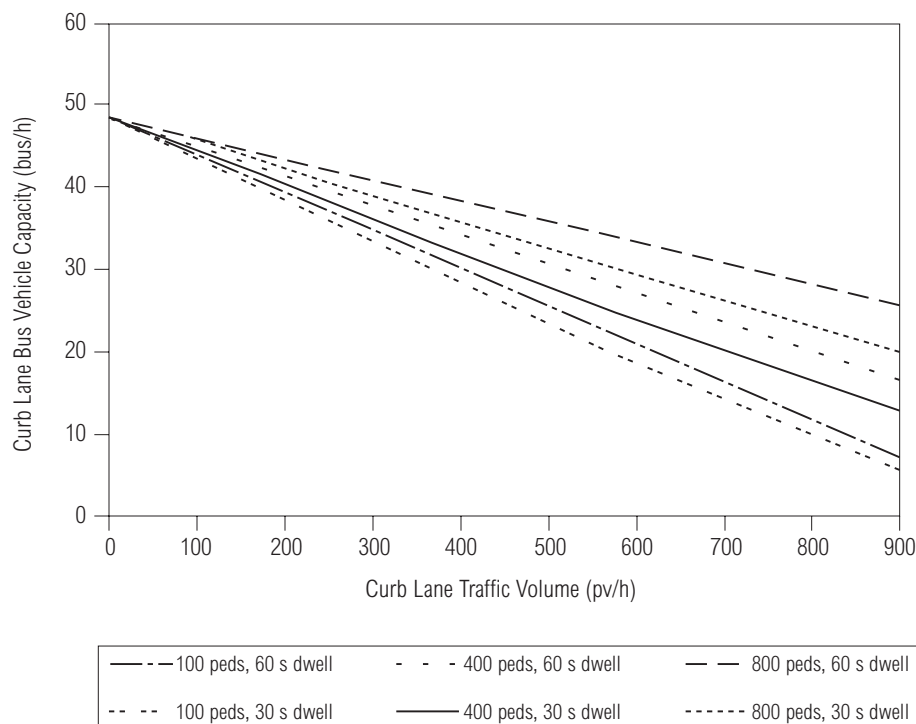
EXHIBIT 14-14. MIXED-TRAFFIC-LANE BUS VEHICLE CAPACITY (SEE FOOTNOTE FOR ASSUMED VALUES)
