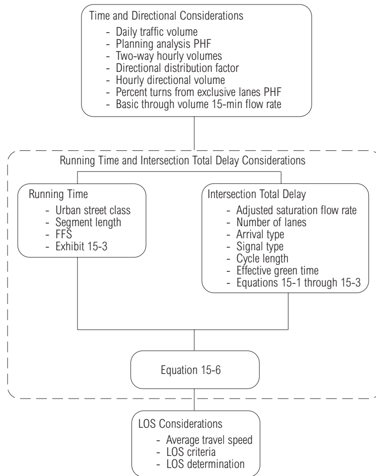
EXHIBIT A15-1. URBAN STREET LOS CALCULATIONS
