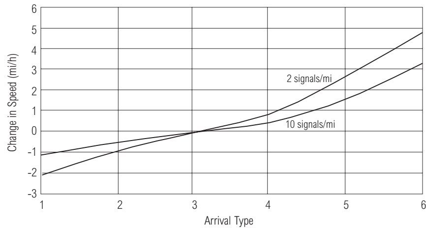
EXHIBIT 15-12. CHANGE IN MEAN SPEED FOR ARRIVAL TYPES (SEE FOOTNOTE FOR ASSUMED VALUES)
