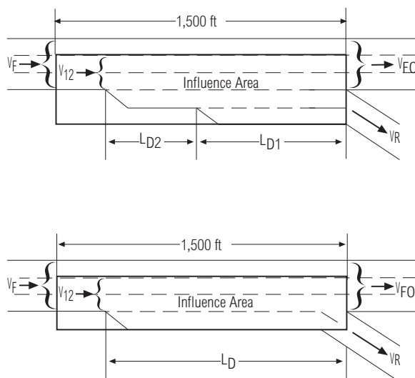
EXHIBIT 25-15. COMMON GEOMETRIES FOR TWO-LANE OFF-RAMPS
