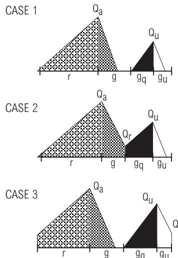
EXHIBIT E16-1. QUEUE ACCUMULATION POLYGONS
