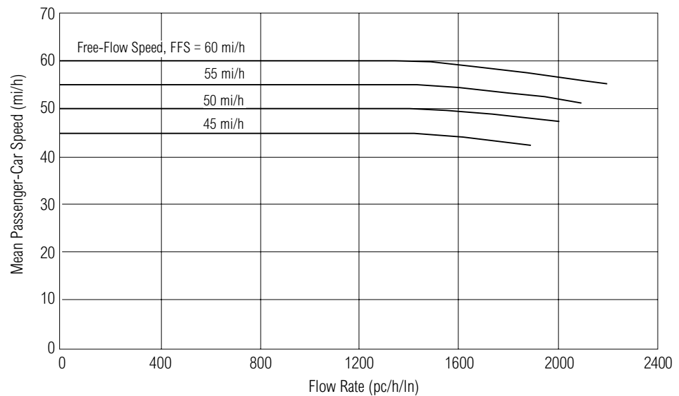
EXHIBIT 12-1. SPEED-FLOW RELATIONSHIPS ON MULTILANE HIGHWAYS
