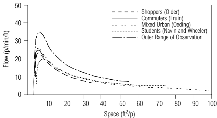
EXHIBIT 11-2. RELATIONSHIPS BETWEEN PEDESTRIAN FLOW AND SPACE
