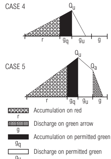
EXHIBIT E16-1. QUEUE ACCUMULATION POLYGONS
