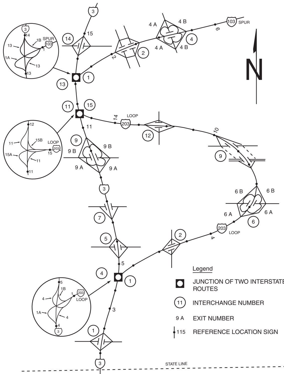
Figure 2E-13. Example of Interchange Numbering for Mainline, Loop, and Spur Routes
